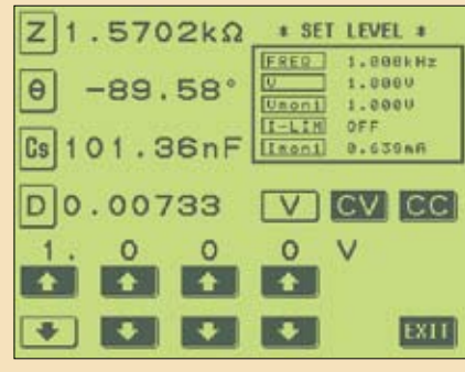
Level setting screens
