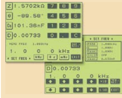
Measurement frequency Use the numeric keypad or digit keys to enter the setting values, changing the test frequency or level while monitoring the measurement. The level setting can be open-circuit voltage, constant voltage, or constant current.
